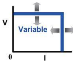
CC+CV Mode
