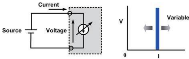
CC Mode
